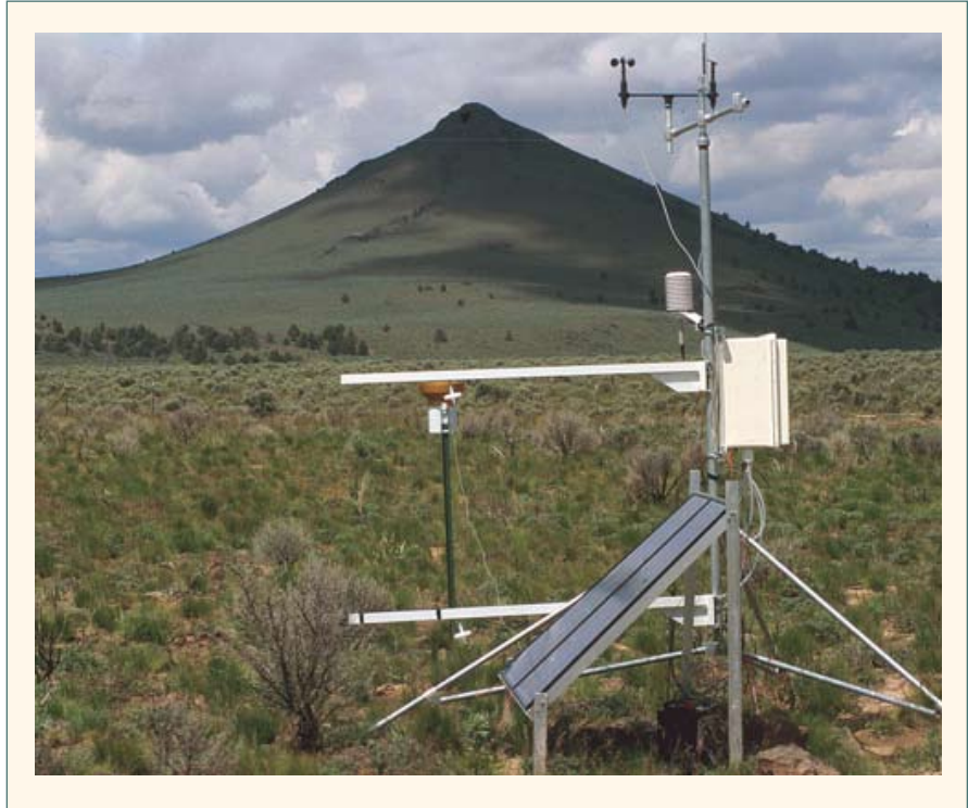
Figure 1. Bowen ratio energy balance instrumentation (Model 023/ \text{CO}_2 , Campbell Scientific, Inc., Logan, Utah, USA)
