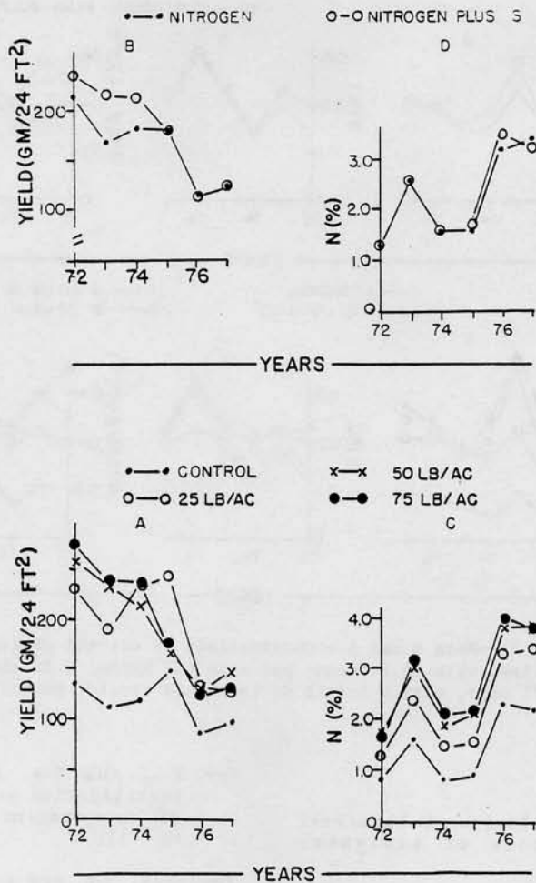
Figure 4.--Mean herbage yield and N concentrations in crested wheatgrass fertilized with 28.5 pounds per acre (32 kg/ha) S in the winter of 1971 only, with N levels as indicated applied annually.
